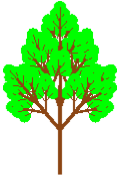
cs1graphics
